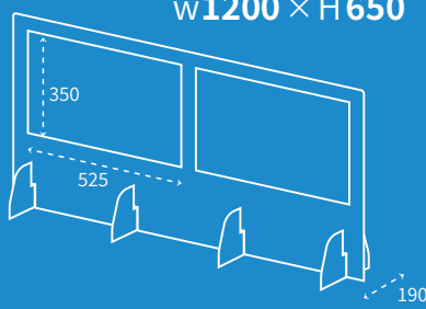
w1200 × H 650
